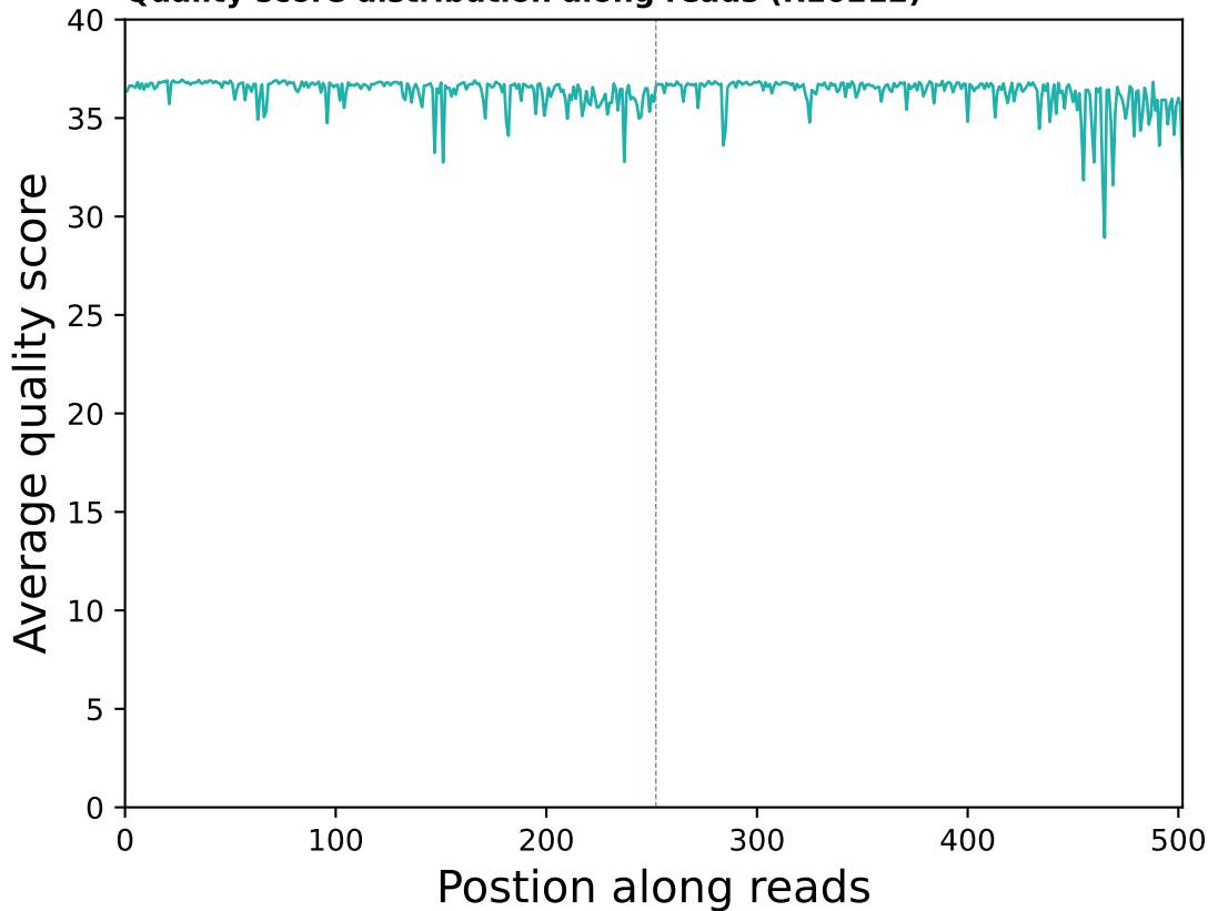
Quality score distribution along reads (R10212)
